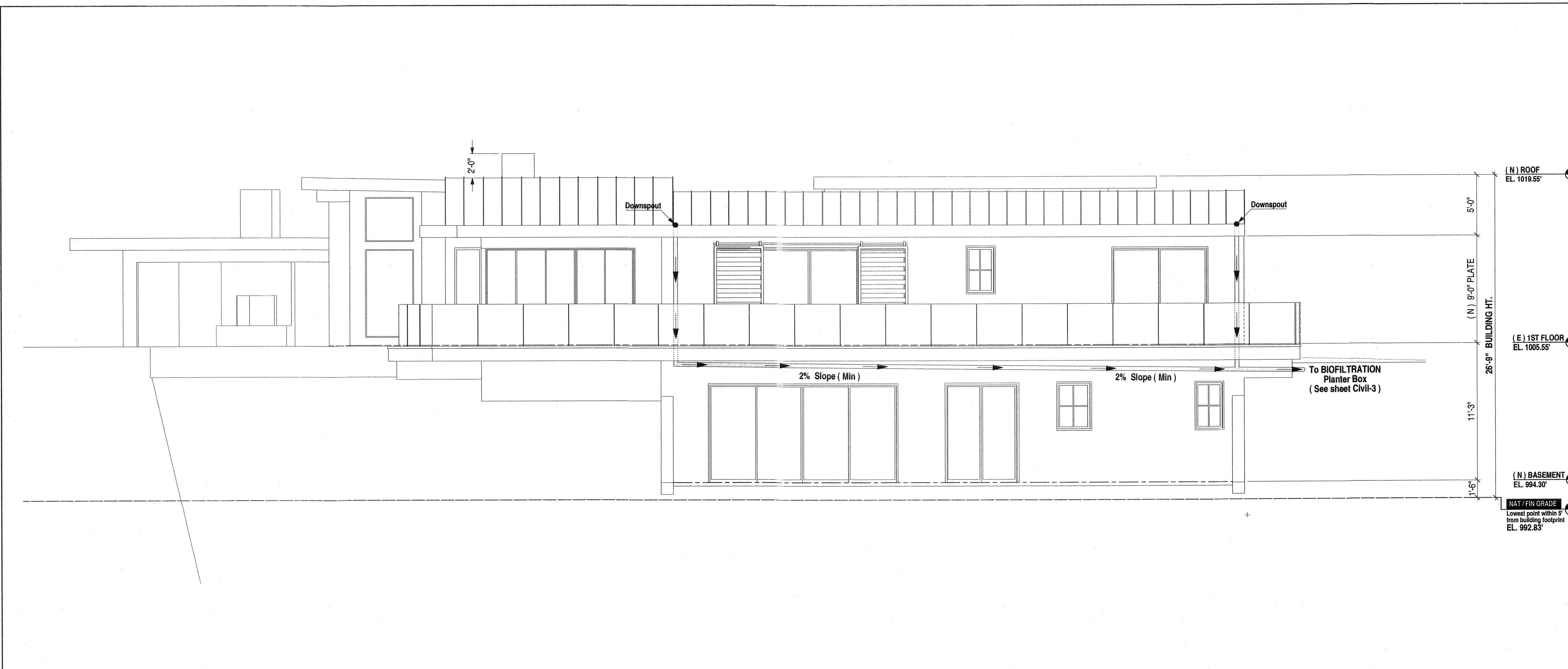
LID ELEVATION - EAST 1 / 4" = 1' - 0"
