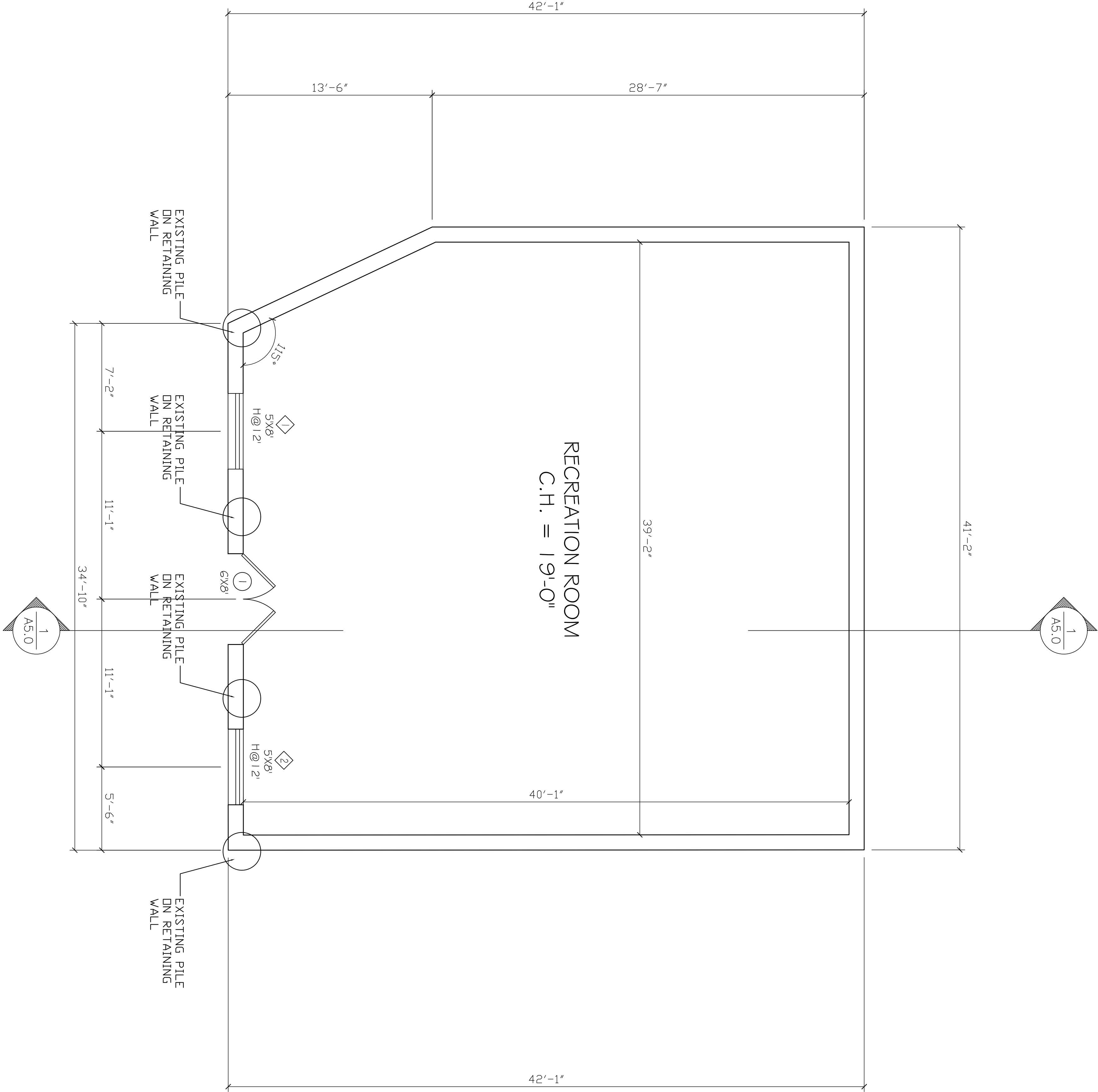
FLOOR PLAN 1/4" = 1'-0"
